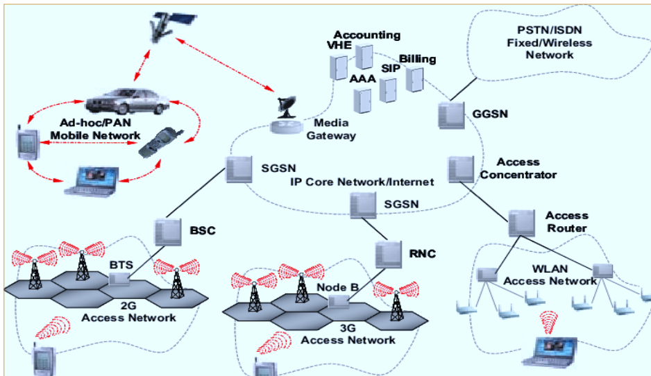
The generic 4G mobile network architecture. Figure (٢):
